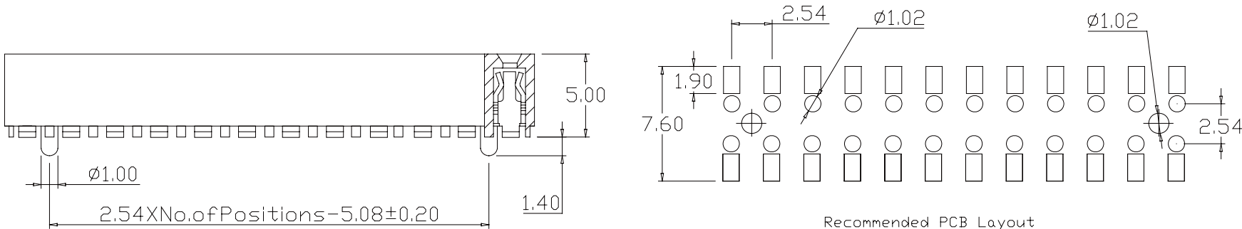
Recommended PCB Layout (PCB TOLERANCE±0.05)
